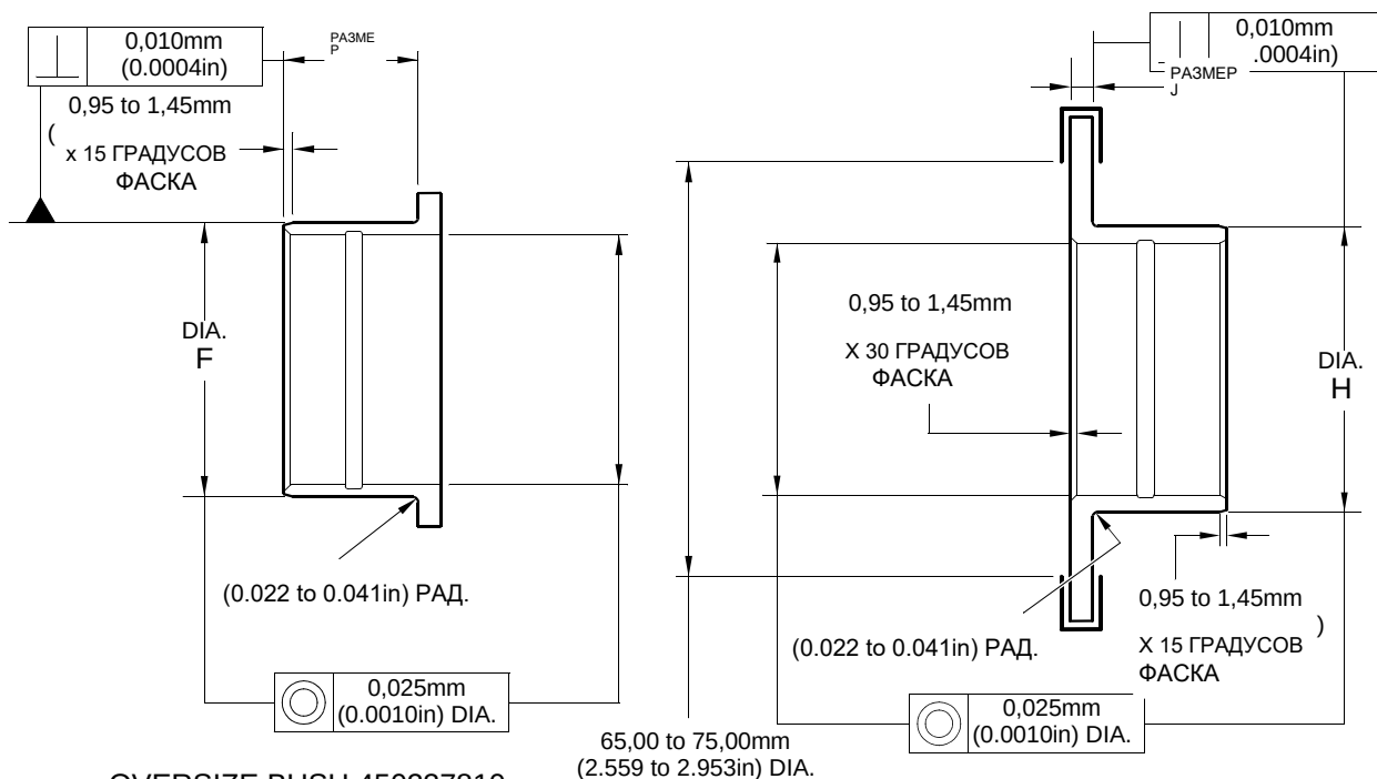
OVERSIZE BUSH 450237810
