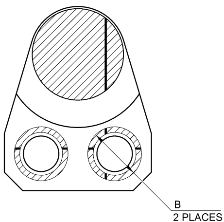
SECTION Z-Z
