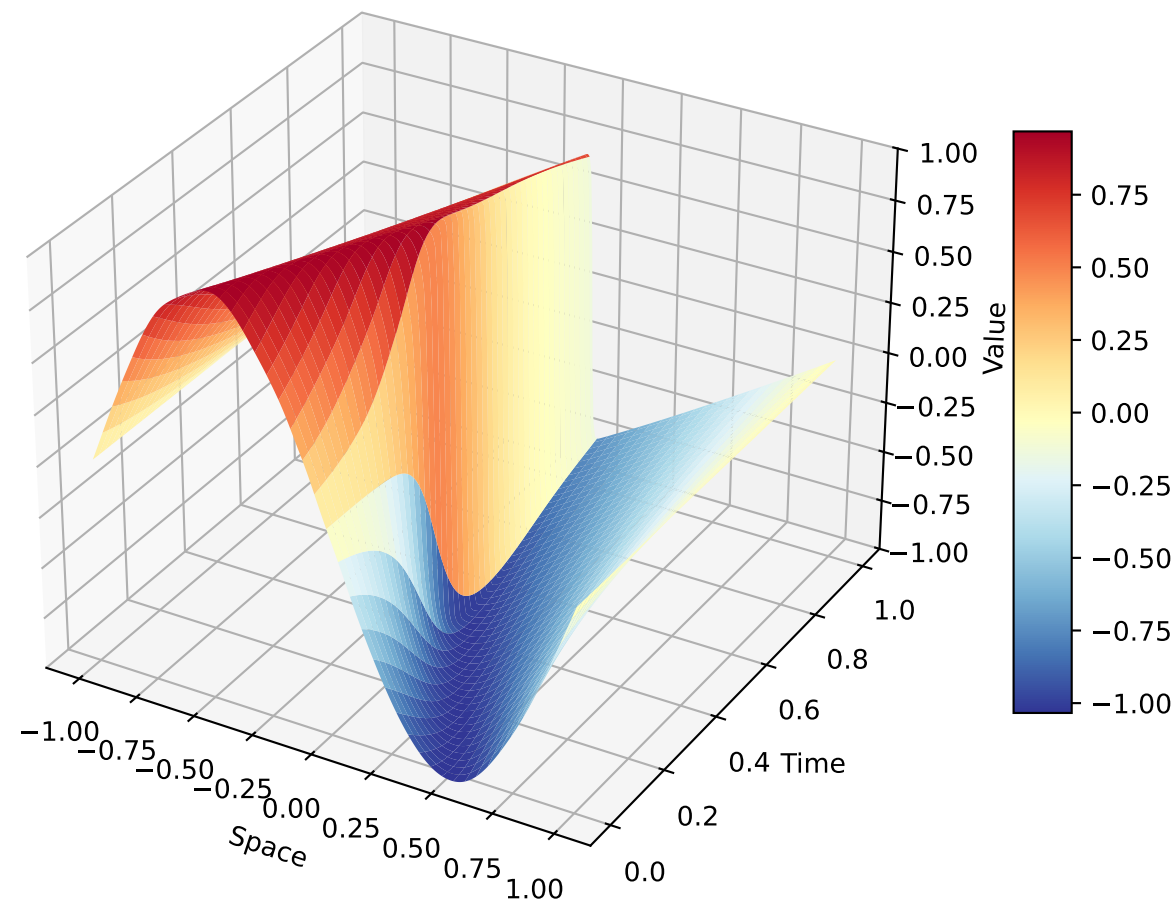
Prediction: KANx[2, 16, 16, 16, 1]
