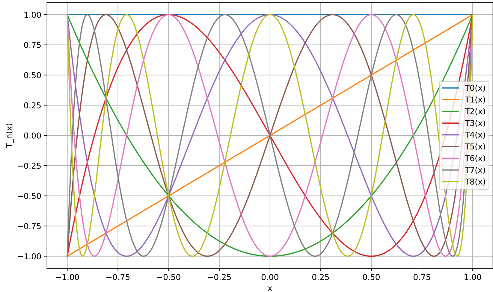
Chebyshev Polynomials on [-1, 1]
