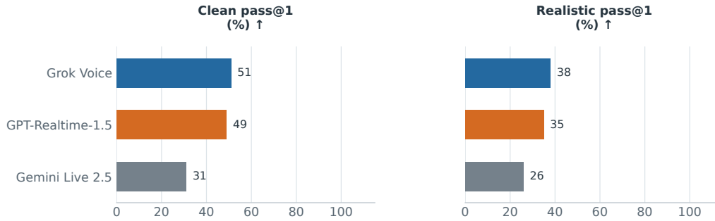
Figure 17: Original \tau -Voice: closed voice references. Units and directions are labeled per panel. Exact values and additional context references are in the adjacent table.
