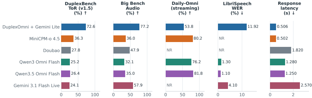
Figure 15: DuplexOmni: streaming/realtime study. Units and directions are labeled per panel. Exact values and additional context references are in the adjacent table.
