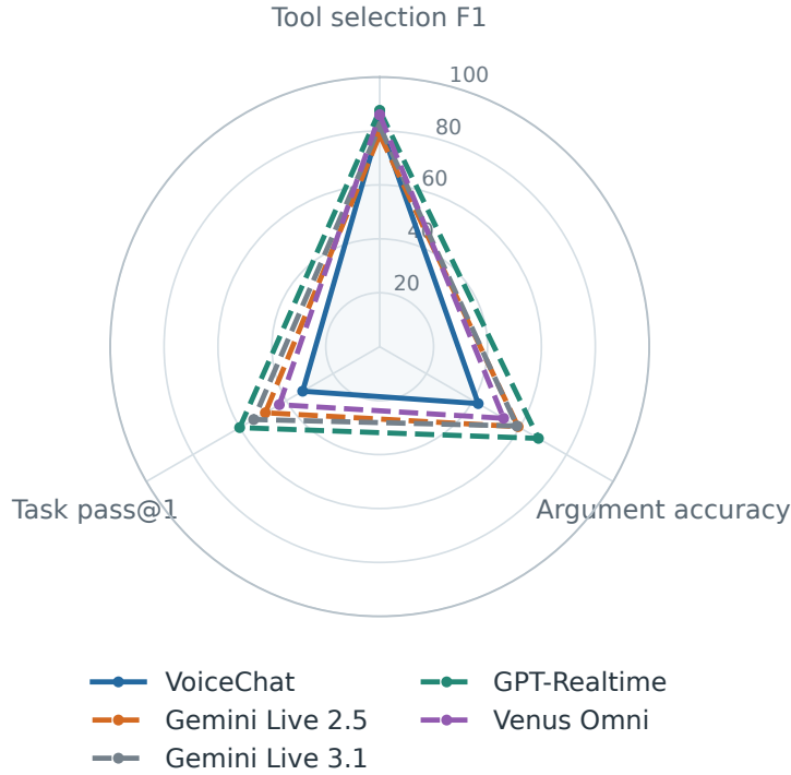
Figure 16: NemotronLabs VoiceChat: Full-Duplex-Bench v3. Raw percentages; higher is better. Exact values and additional context references are in the adjacent table.
