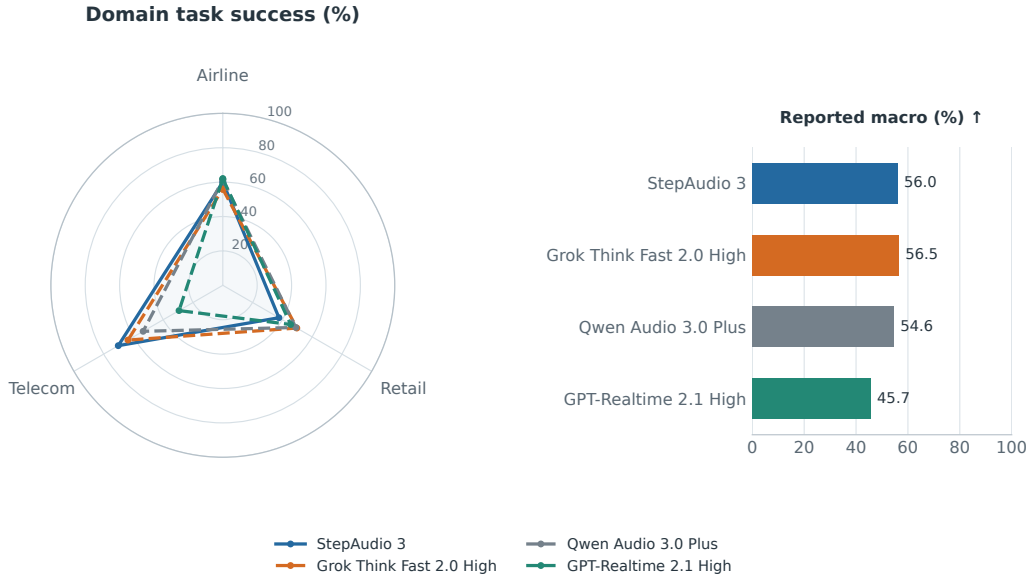
Figure 12: StepAudio 3 Realtime: \tau -Voice (AA). Raw percentages; higher is better. Exact values and additional context references are in the adjacent table.
