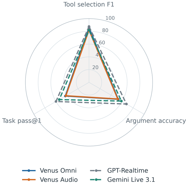
Figure 13: Realtime-Venus: Full-Duplex-Bench v3. Raw percentages; higher is better. Exact values and additional context references are in the adjacent table.
