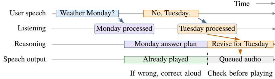
Figure 19: Illustrative Monday-to-Tuesday correction, not an experimental result. User speech may enter as audio tokens or acoustic features. Once the correction is processed, revise the answer plan and check queued audio before playback. Wrong claims already played need an audible correction; they cannot be taken back.
