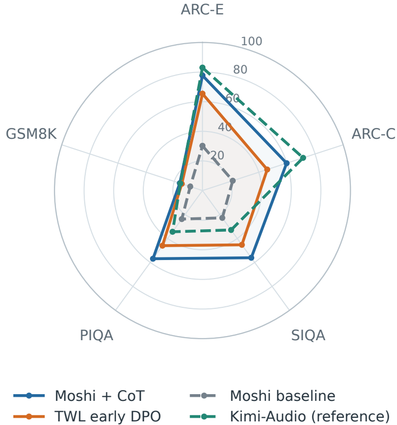
Figure 9: Think while listening: SRQA. Raw percentages; higher is better. Exact values and additional context references are in the adjacent table.
