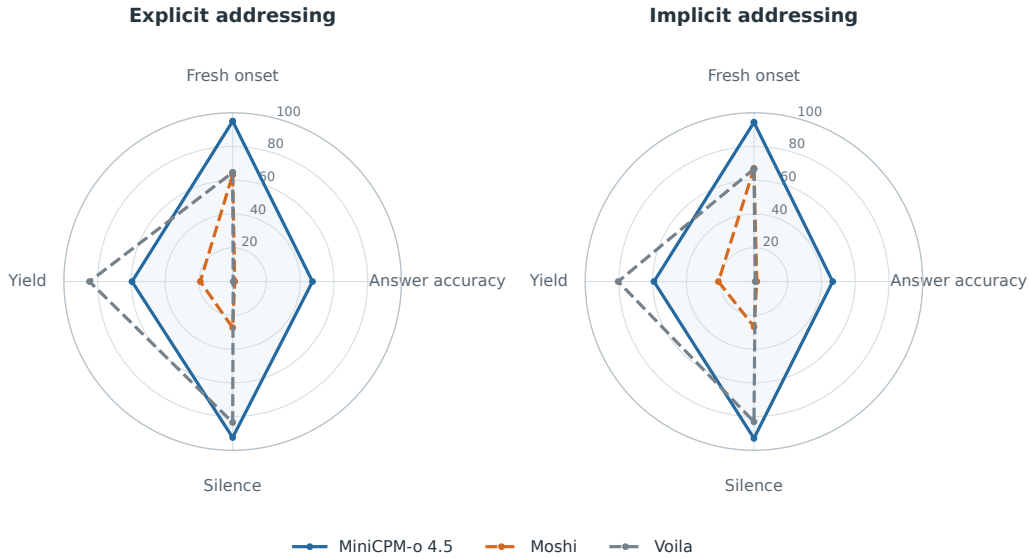
Figure 14: MiniCPM-o 4.5: Duplex-MPE. Raw percentages; higher is better. Exact values and additional context references are in the adjacent table.
