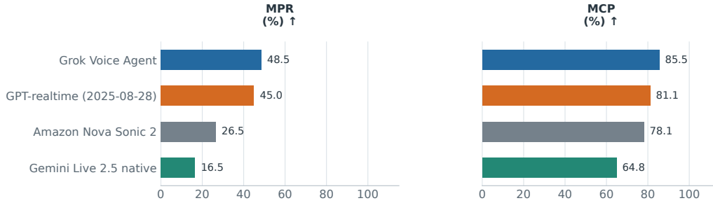
Figure 18: EchoChain: closed voice references. Units and directions are labeled per panel. Exact values and additional context references are in the adjacent table.
