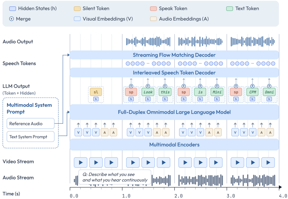
Figure 2: MiniCPM-o 4.5 . Reproduced from Cui et al. (2026), Fig. 4. A timed Qwen3-8B text backbone receives streaming multimodal input; separate speech-token and waveform decoders render its response. Open inference does not imply release of the complete training mixture.
