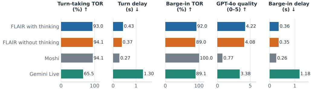
Figure 11: FLAIR: earlier duplex interaction suite. Units and directions are labeled per panel. Exact values and additional context references are in the adjacent table.
