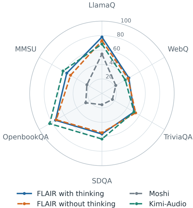
Figure 10: FLAIR: spoken QA accuracy. Raw percentages; higher is better. Exact values and additional context references are in the adjacent table.
