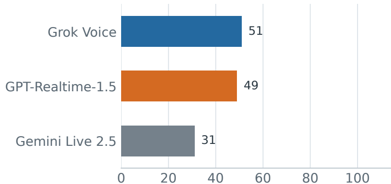
Clean pass@1 (%) ↑
