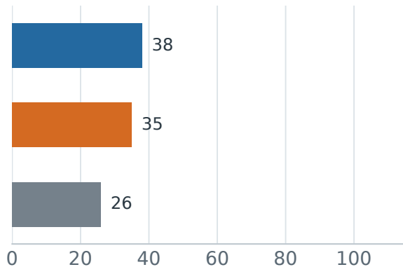
Realistic pass@1 (%) ↑
