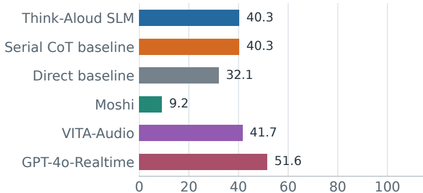
WebQuestions (%) ↑
