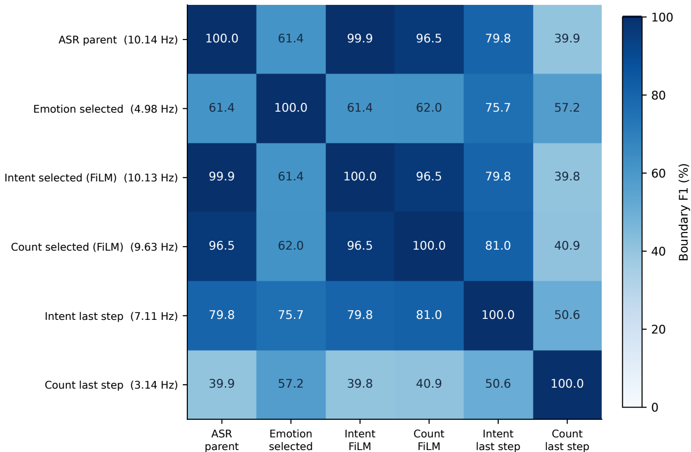
Expresso: agreement of different task checkpoints One-to-one boundary F1 at \pm 20 ms; seed 3408, 420 identical utterances
