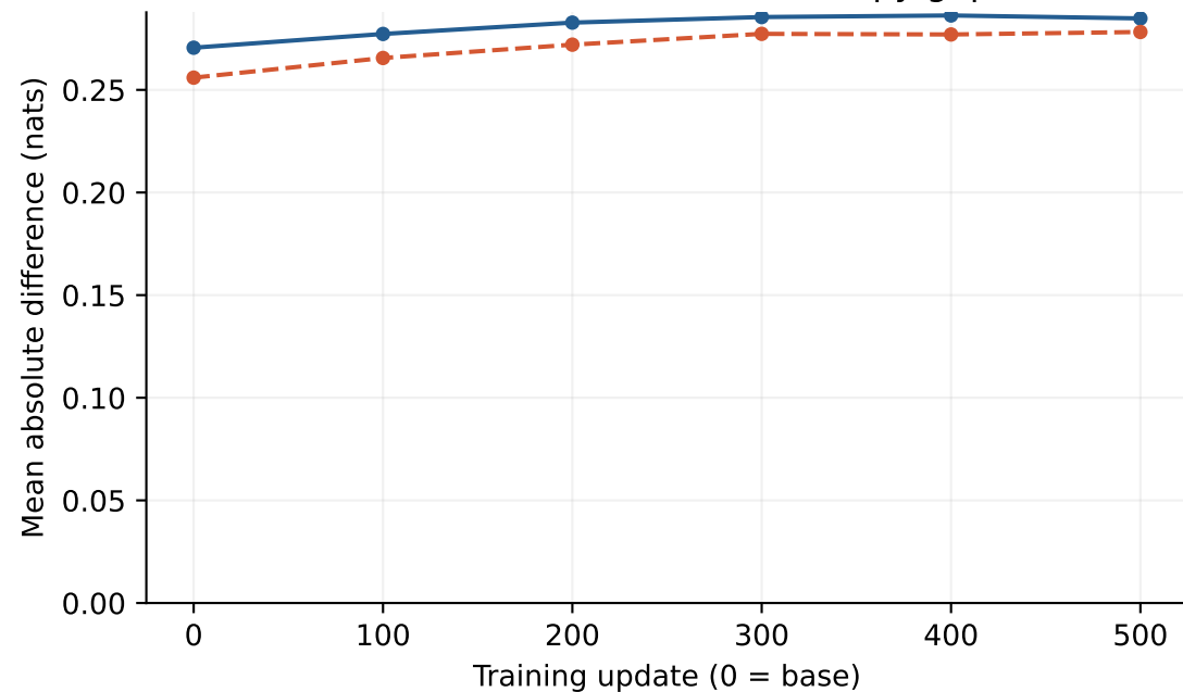
C. Same-model absolute entropy gap
