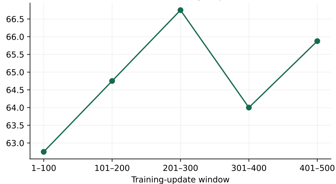
Logged periodic-reference absolute entropy gap (nats)
