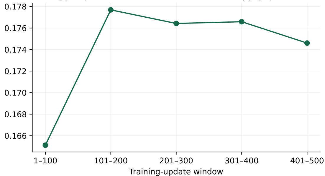
Logged periodic-reference absolute entropy gap (nats)
