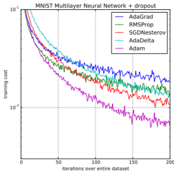
Figure 4.13: Comparison between AdaGrad, RMSProp, SGD Nesterov, AdaDelta and Adam
