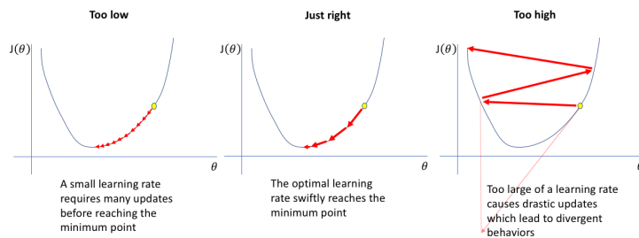
Figure 4.18: Learning Rate explained
