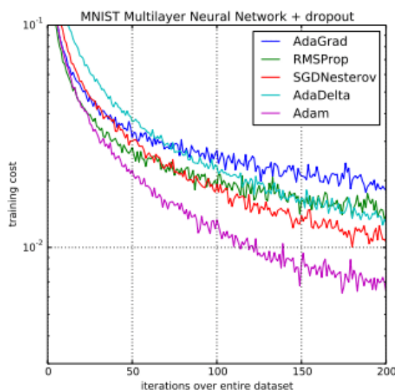
Figure 4.17: Comparison between AdaGrad, RMSProp, SGD Nesterov, AdaDelta and Adam
