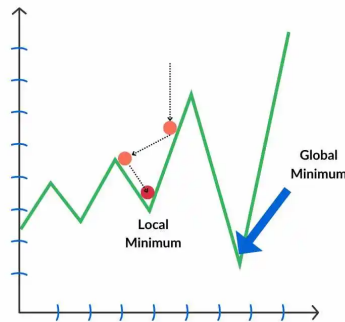
Figure 4.16: Stochastic Gradient Descent
