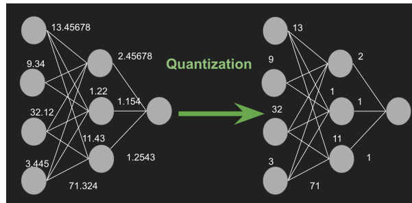
Figure 4.14: Quantization
