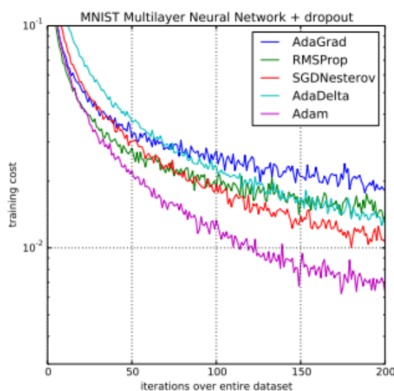
Figure 4.12: Comparison between AdaGrad, RMSProp, SGD Nesterov, AdaDelta and Adam
