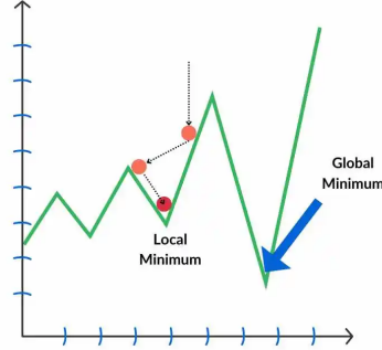
Figure 4.11: Stochastic Gradient Descent
