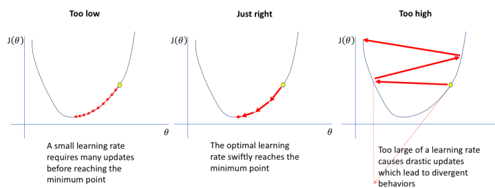
Figure 4.13: Learning Rate explained
