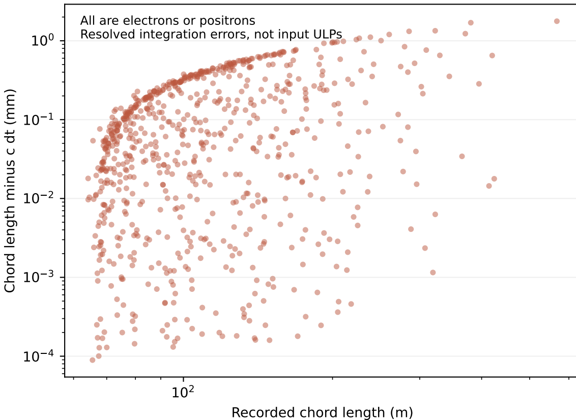
Actual 100 PeV air-shower failure: 766 sources
