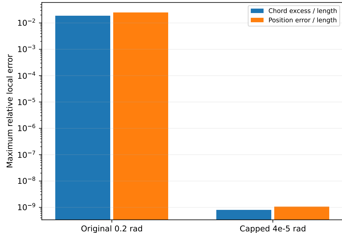
Independent exact helix: both charge signs / fields / pitches
