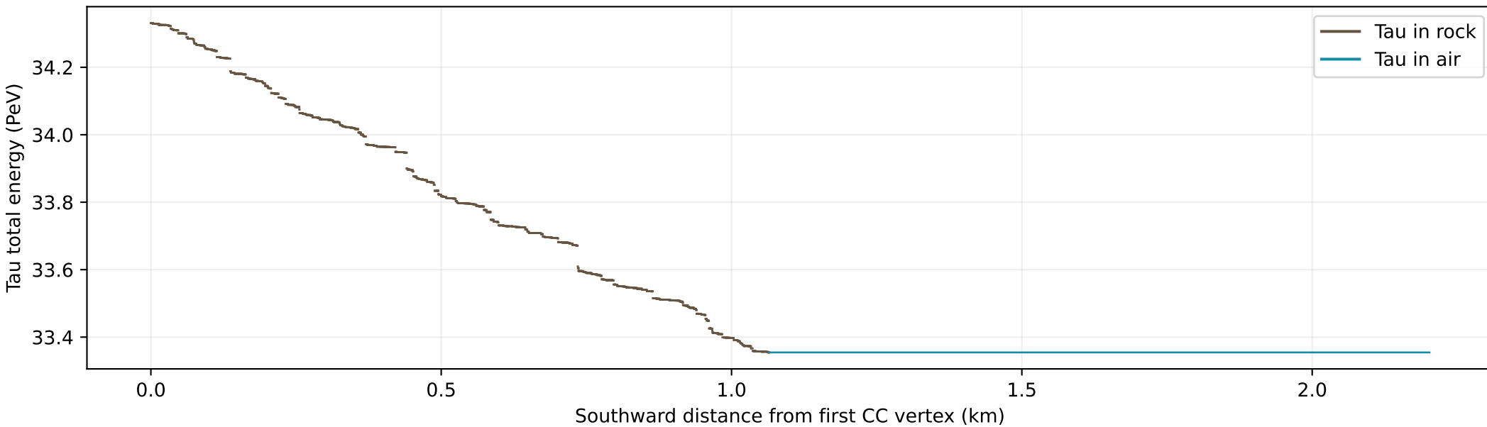
Actual transport energy loss; no fitted decay position
