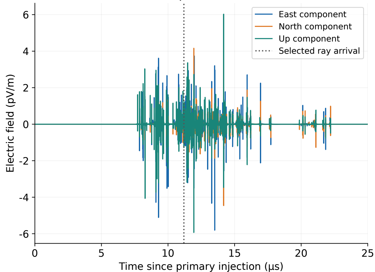
Actual three-component waveform at E01
