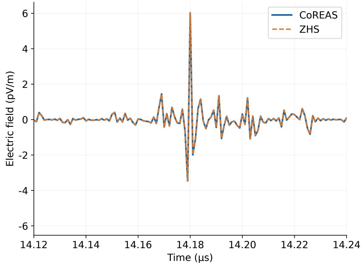
E01 pulse: same field component
