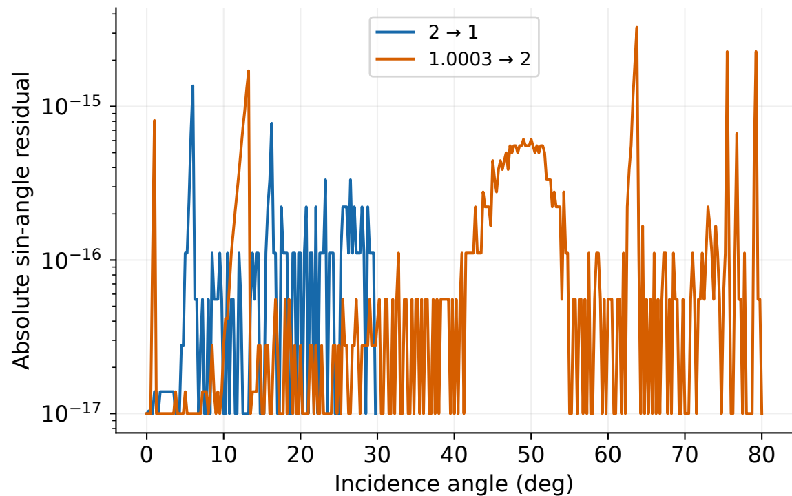
Identical TIR classification: 642 / 642
