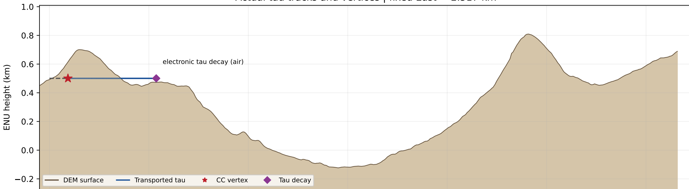
Silica (SiO 2 ) | seed 946 | 100 PeV nu tau Actual tau tracks and vertices | fixed East = 2.517 km
