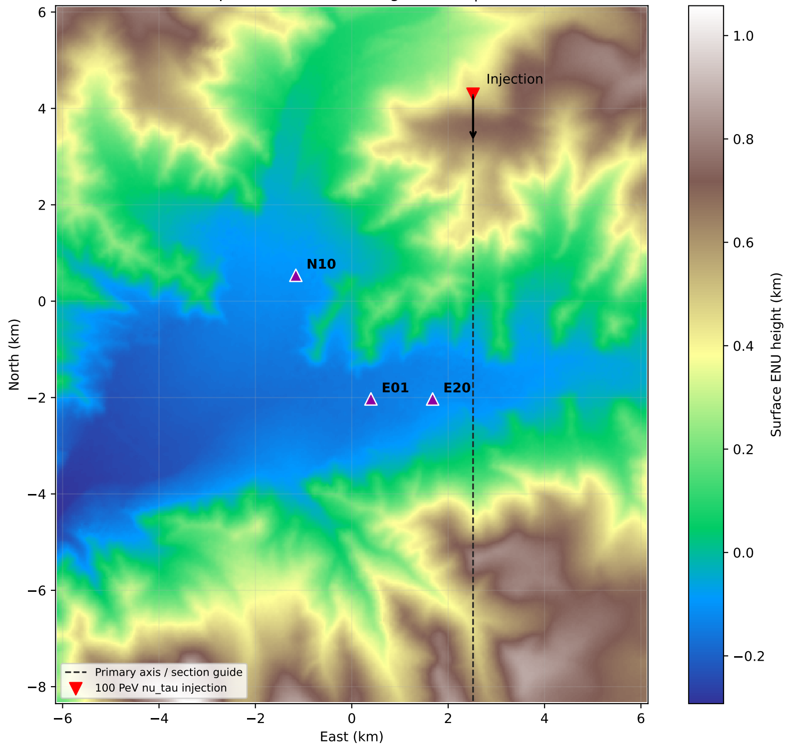
Common input DEM and receiving stations | all 9 events
