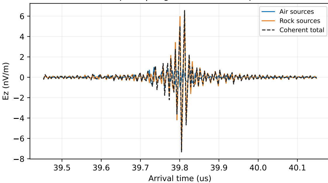
Near air peak | original time and amplitude
