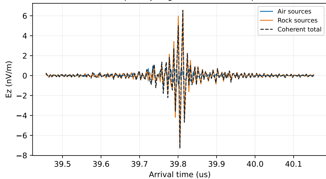
Near rock peak | original time and amplitude
