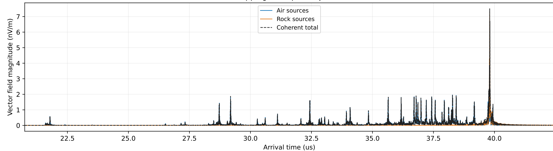
Near air peak | original time and amplitude
