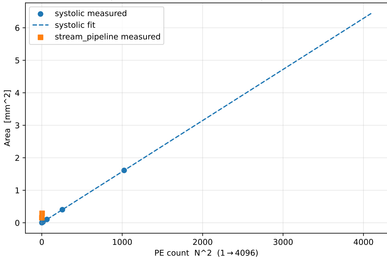
M3 sweep: area vs. PE count, fit + extrapolation to 64x64
