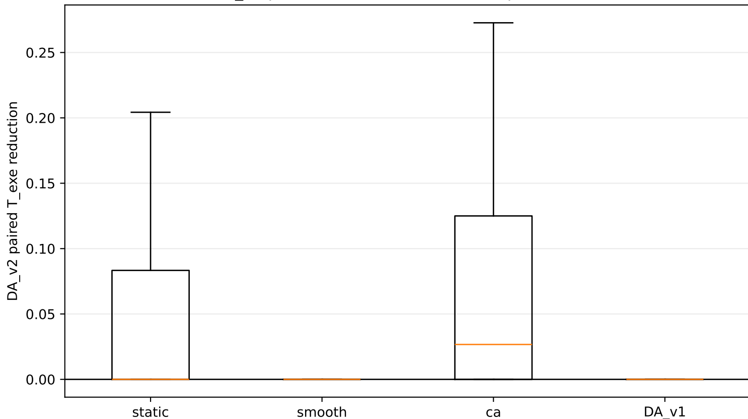
DA_v2 paired executable-runtime improvements
