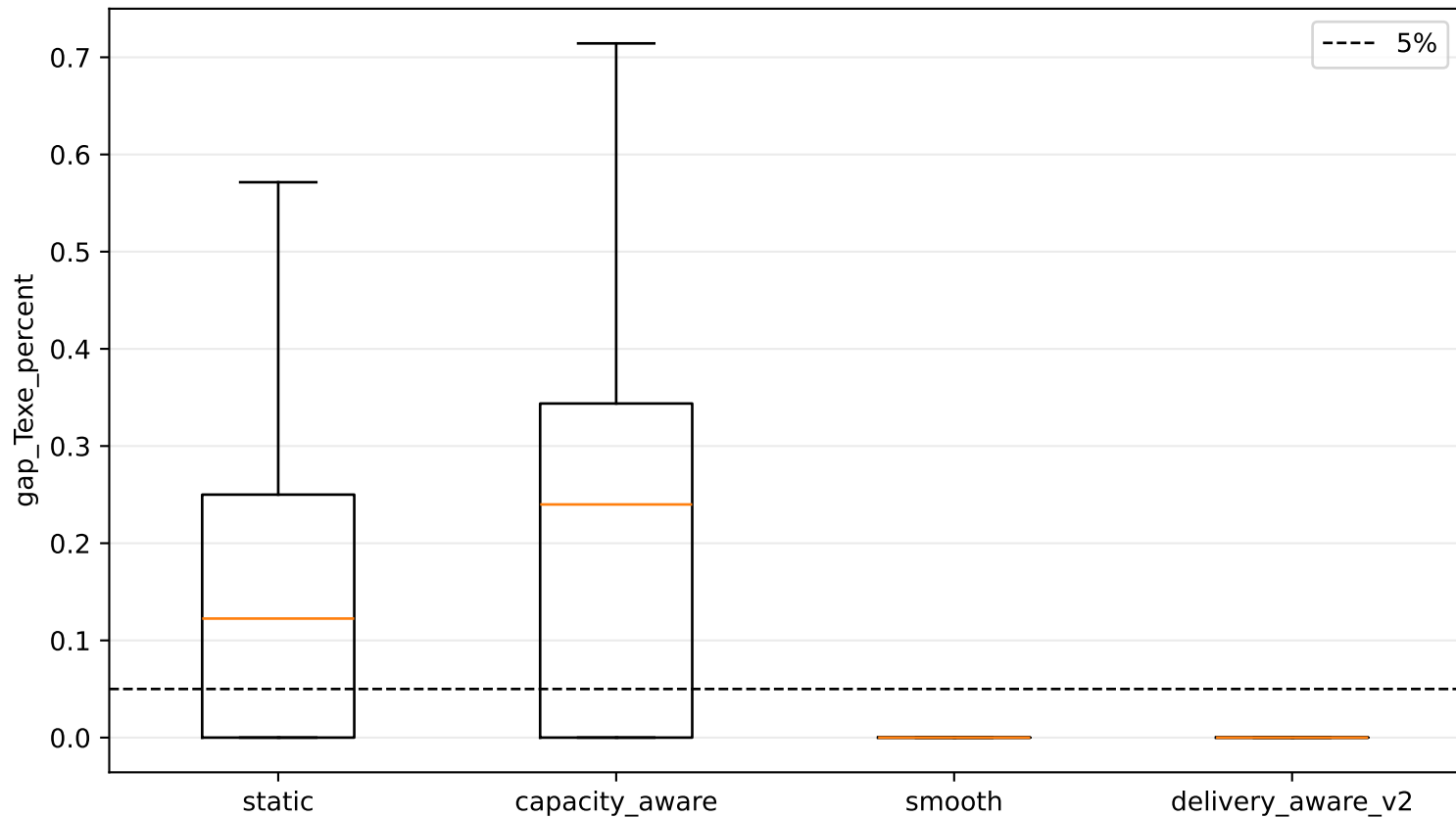
Gap to near-optimal deterministic reference
