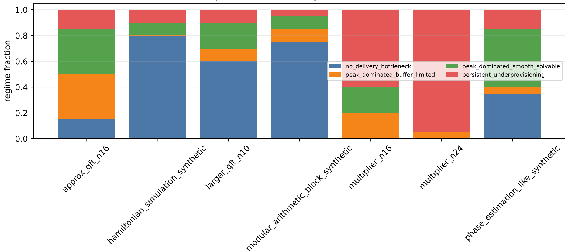
Expanded workload regime distribution
