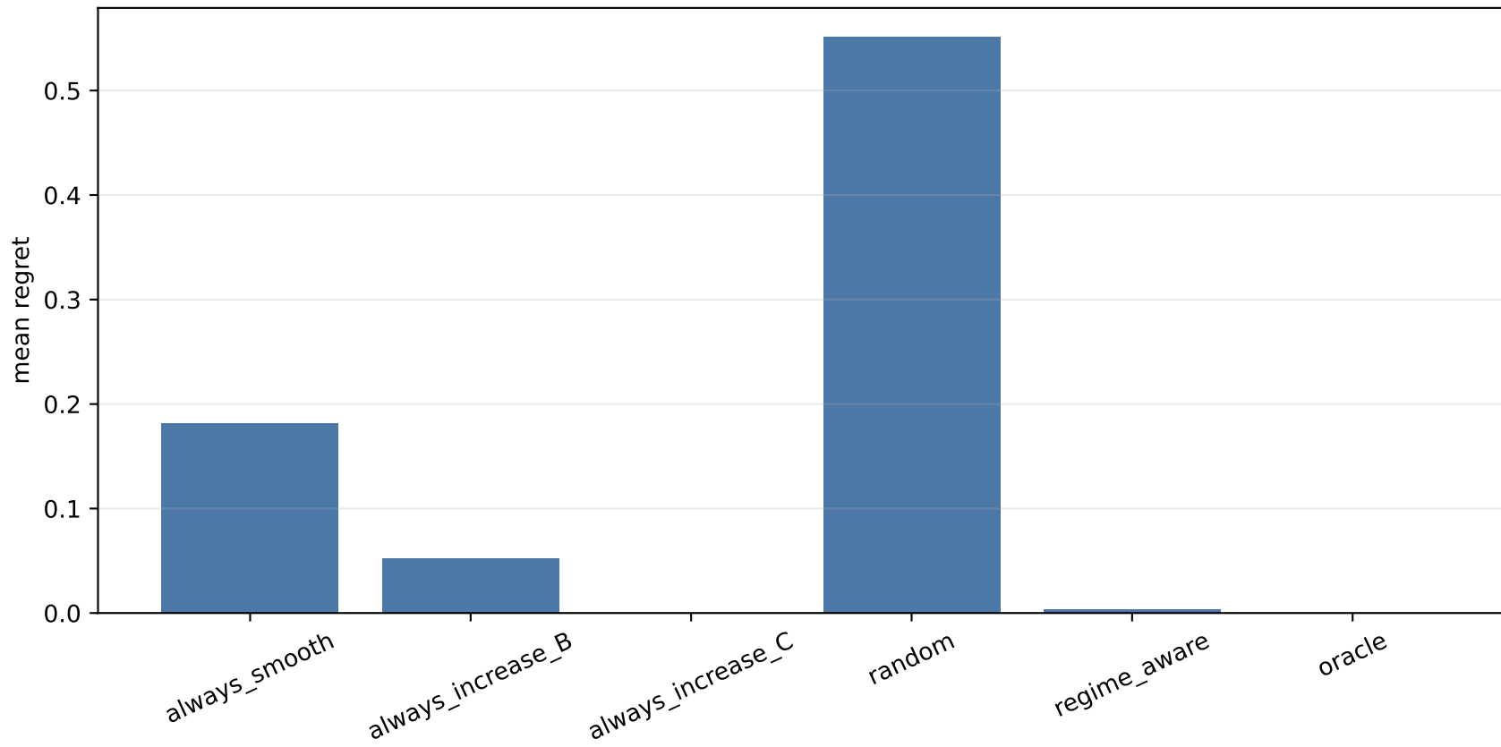
Policy baseline comparison
