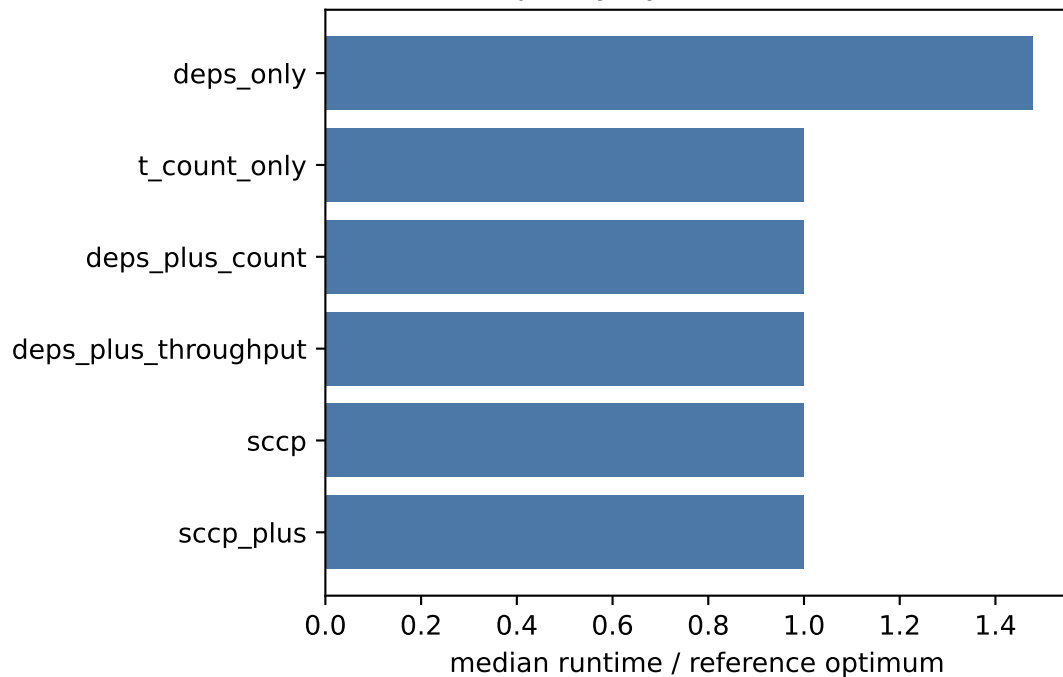
Selection quality by cost-model information
