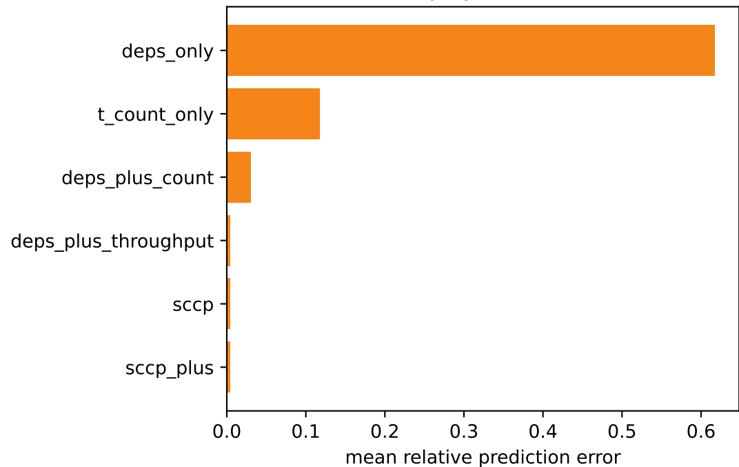
Prediction accuracy by cost-model information
