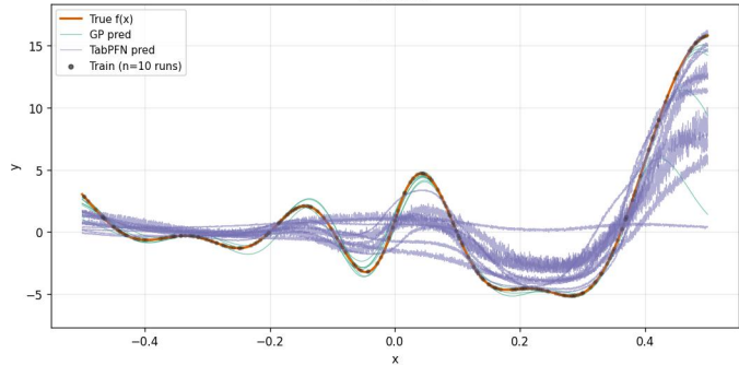
A22_damped_forrester_1Dx_20Dn_[-0.5,0.5]_16inits_noiseTest0.0_noiseTrain0.0_x10 all 10 runs
