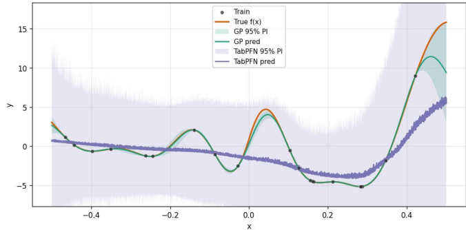
A22_damped_forrester_1Dx_20Dn_ [-0.5, 0.5] _16inits_noiseTest0.0_noiseTrain0.0_x10 run 1
