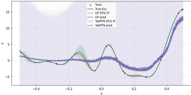
A22_damped_forrester_1Dx_20Dn_ [-0.5, 0.5] _16inits_noiseTest0.0_noiseTrain0.0_x10 run 2
