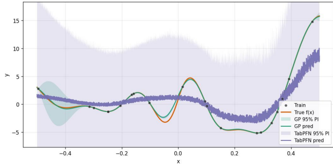
A22_damped_forrester_1Dx_20Dn_ [-0.5, 0.5] _16inits_noiseTest0.0_noiseTrain0.0_x10 run 5
