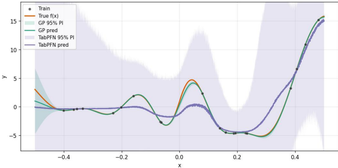
A22_damped_forrester_1Dx_20Dn_ [-0.5, 0.5] _16inits_noiseTest0.0_noiseTrain0.0_x10 run 7
