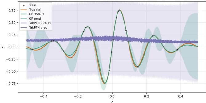
A22_damped_sine_1Dx_20Dn_ [-0.5, 0.5]_{16} inits_noiseTest0.0_noiseTrain0.0_x10 run 10
