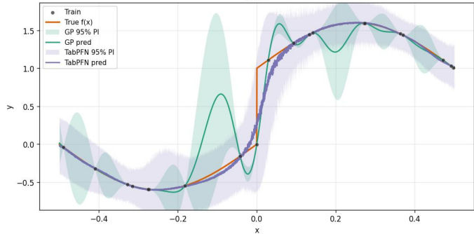
A22_discontinuity_1Dx_20Dn_ [-0.5,0.5] _16inits_noiseTest0.0_noiseTrain0.0_x10 run 2
