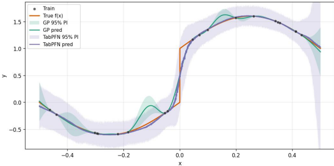
A22_discontinuity_1Dx_20Dn_ [-0.5,0.5] _16inits_noiseTest0.0_noiseTrain0.0_x10 run 3
