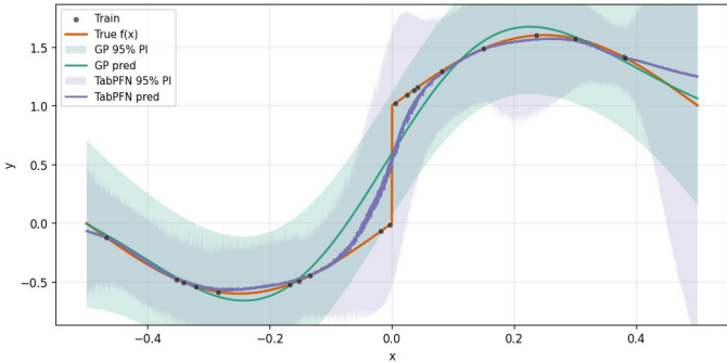
A22_discontinuity_1Dx_20Dn_ [-0.5, 0.5] _16inits_noiseTest0.0_noiseTrain0.0_x10 run 10
