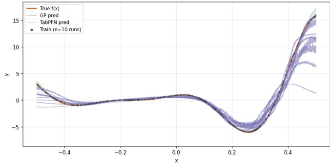
A22_forrester_1Dx_20Dn_ [-0.5, 0.5] _16inits_noiseTest0.0_noiseTrain0.0_x10 all 10 runs
