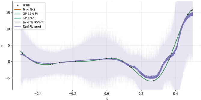
A22_forrester_1Dx_20Dn_ [-0.5, 0.5]_{16} inits_noiseTest0.0_noiseTrain0.0_x10 run 2
