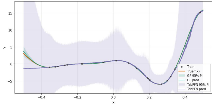
A22_forrester_1Dx_20Dn_ [-0.5, 0.5] _16inits_noiseTest0.0_noiseTrain0.0_x10 run 8
