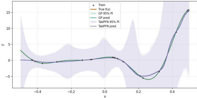
A22_forrester_1Dx_20Dn_ [-0.5, 0.5]_{16} inits_noiseTest0.0_noiseTrain0.0_x10 run 9
