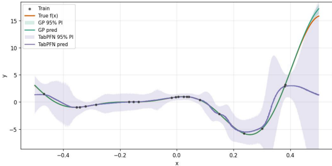
A22_forrester_1Dx_20Dn_ [-0.5, 0.5] _16inits_noiseTest0.0_noiseTrain0.0_x10 run 10
