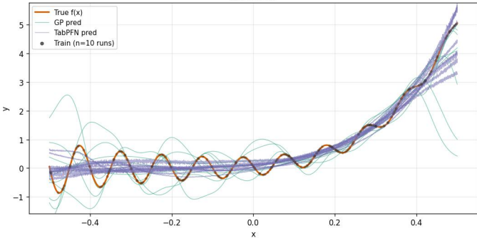
A22_gramacy_lee_1Dx_20Dn_ [-0.5, 0.5] _16inits_noiseTest0.0_noiseTrain0.0_x10 all 10 runs
