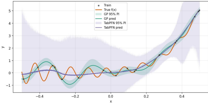
A22_gramacy_lee_1Dx_20Dn_ [-0.5, 0.5] _16inits_noiseTest0.0_noiseTrain0.0_x10 run 2
