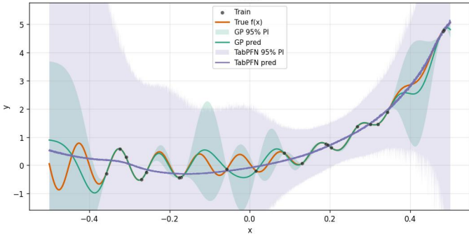
A22_gramacy_lee_1Dx_20Dn_ [-0.5, 0.5] _16inits_noiseTest0.0_noiseTrain0.0_x10 run 8
