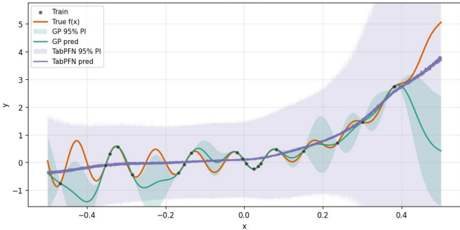
A22_gramacy_lee_1Dx_20Dn_ [-0.5, 0.5] _16inits_noiseTest0.0_noiseTrain0.0_x10 run 10
