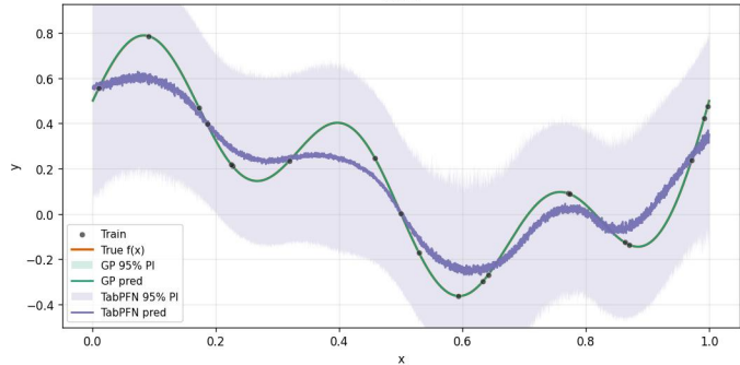
A22_sin_cubic_1Dx_20Dn_[0.0,1.0]_16inits_noiseTest0.0_noiseTrain0.0_x10 run 2
