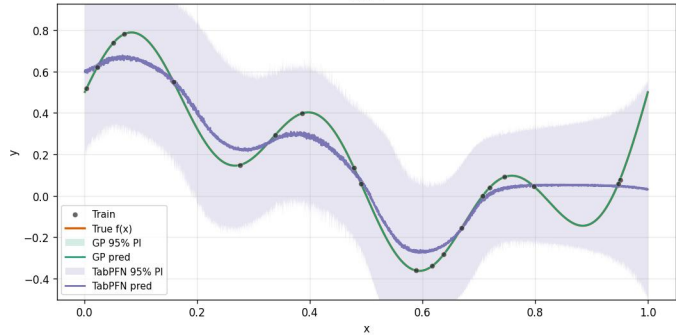
A22_sin_cubic_1Dx_20Dn_[0.0,1.0]_16inits_noiseTest0.0_noiseTrain0.0_x10 run 4
