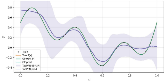
A22_sin_cubic_1Dx_20Dn_[0.0,1.0]_16inits_noiseTest0.0_noiseTrain0.0_x10 run 6
