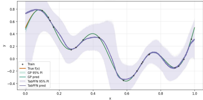
A22_sin_cubic_1Dx_20Dn_[0.0,1.0]_16inits_noiseTest0.0_noiseTrain0.0_x10 run 7
