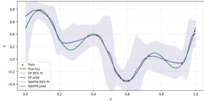
A22_sin_cubic_1Dx_20Dn_[0.0,1.0]_16inits_noiseTest0.0_noiseTrain0.0_x10 run 9
